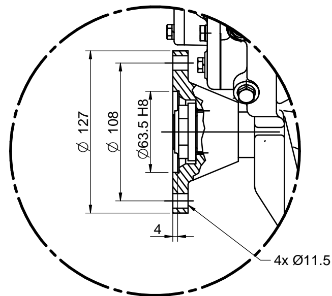
Detalle/Detail A
