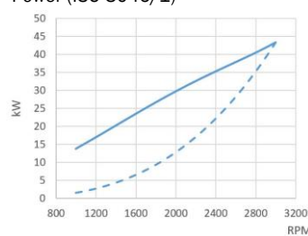
Power (ISO 3046/1)
