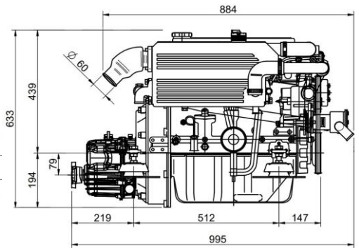
MINI-62 Engine TMC-60P 2.00:1 Gbox.
