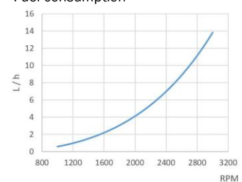
Fuel consumption
