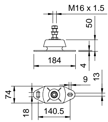
Supensor/Engine Mount
