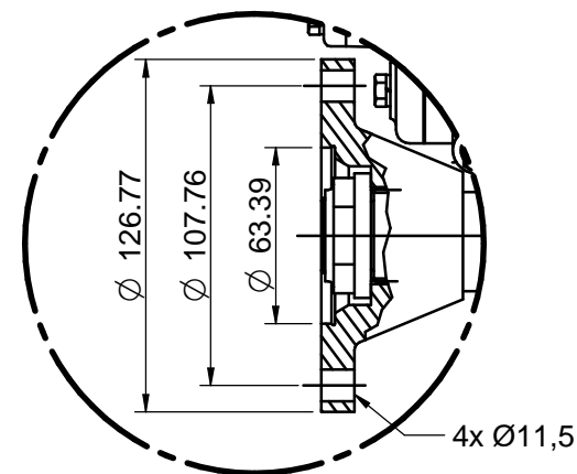
Detalle/Detail A
