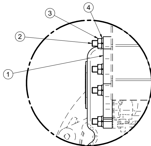
Detalle/Detail A
