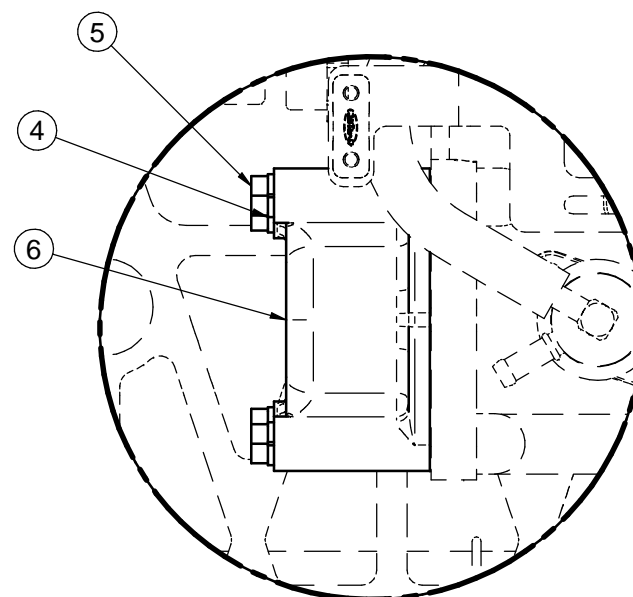
Detalle/Detail B
