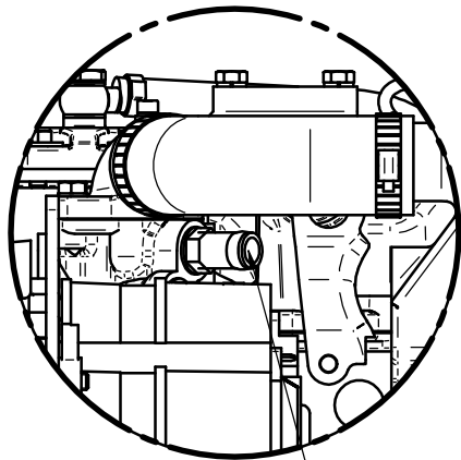
Entrada/Inlet Ø17,5mm
