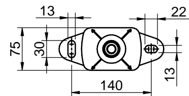
Supensor/Engine Mount
