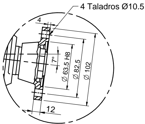
Detalle/Detail A
