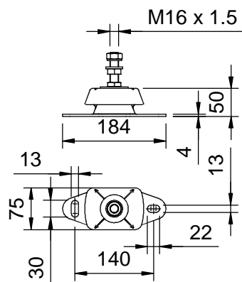
Supensor/Engine Mount
