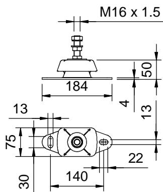
Supensor/Engine Mount
