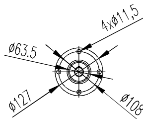
BRIDA INVERSOR/COUPLING GEARBOX
