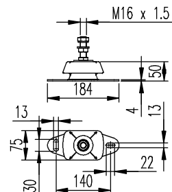
Supensor/Engine Mount
