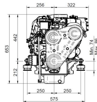
Motor SK-60 Inv.TMC-60P 2,00:1
