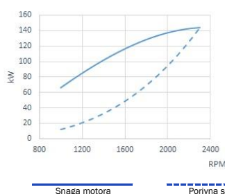
Snaga (ISO 3046/1)
