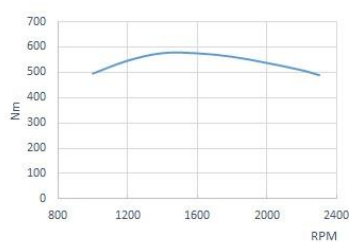
Crankshaft torque
