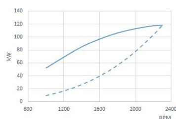
Power (ISO 3046/1)
