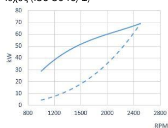
Ισχύς (ISO 3046/1)
