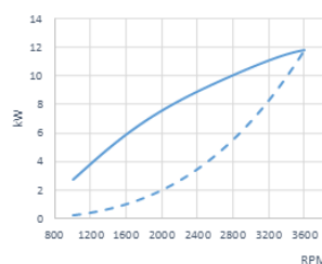
Vermogen (ISO 3046/1)
