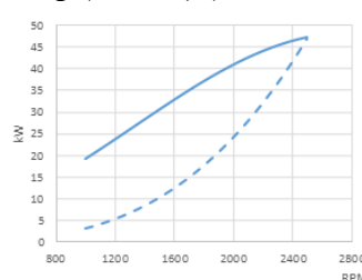
Snaga (ISO 3046/1)
