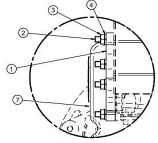
Detalle/Detail A
